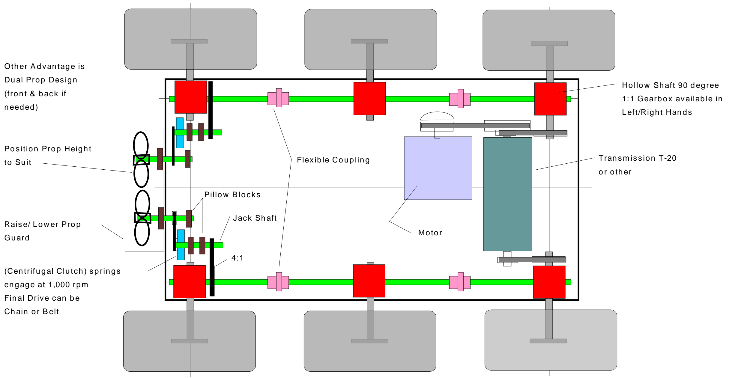
SCHMATIC OF CLUTCHED PROPS with dual prop design
