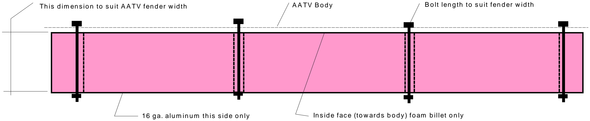
TOP VIEW
