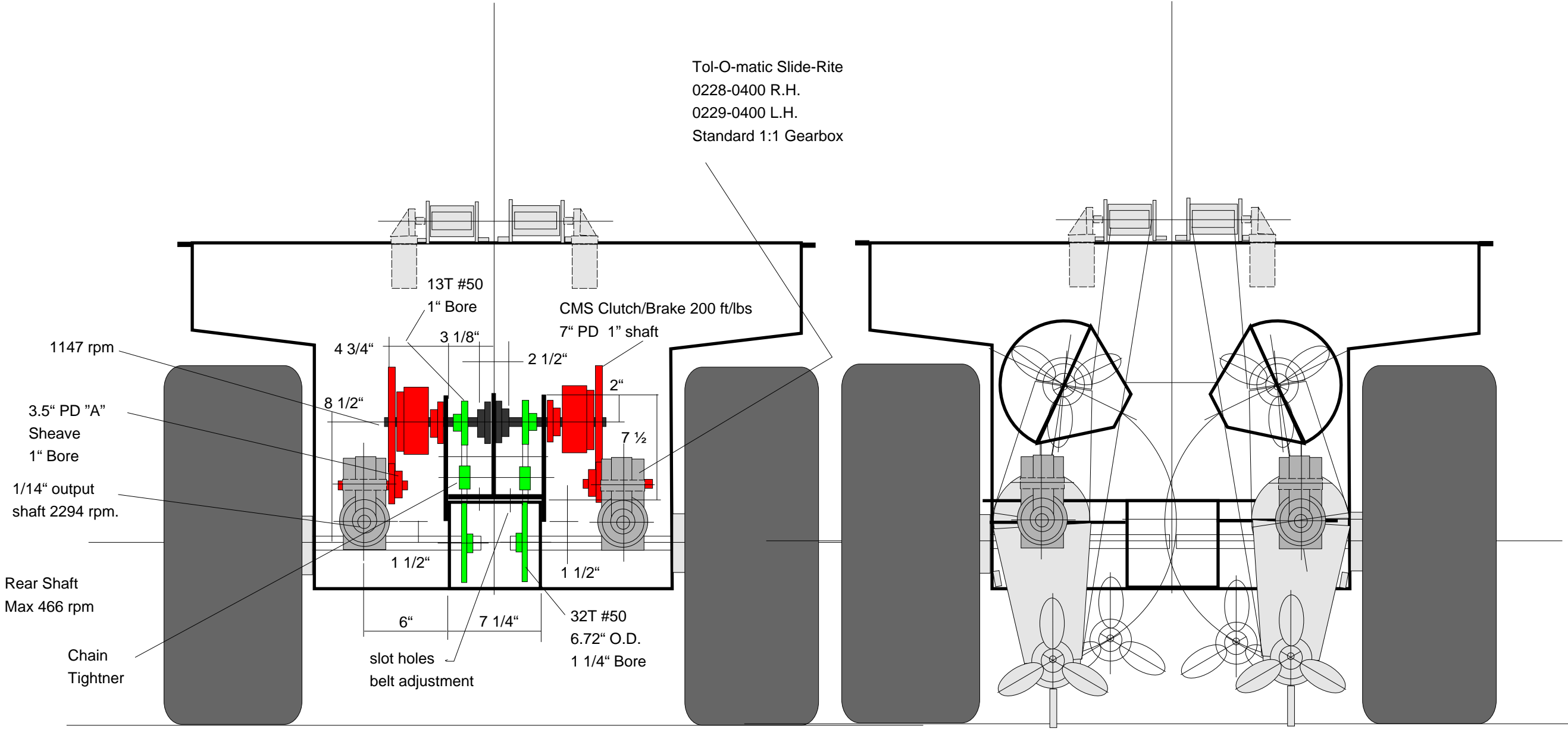
Dual Prop Outdrive
